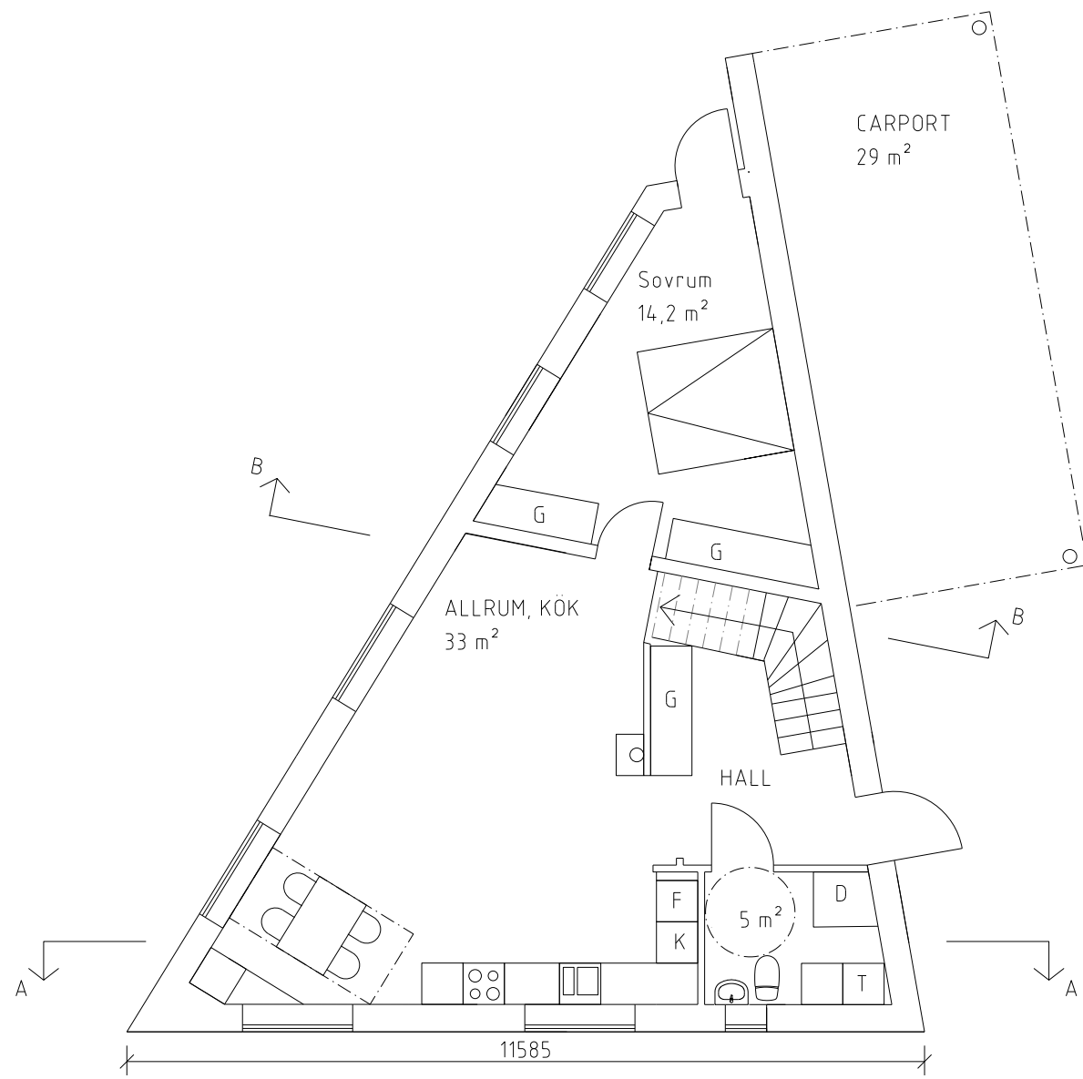
MARKPLAN
