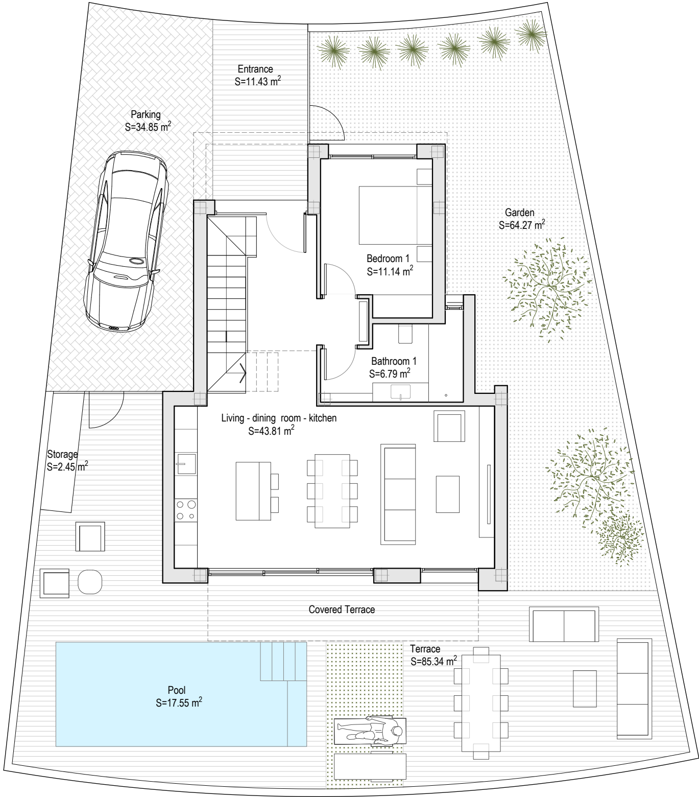
Ground floor
