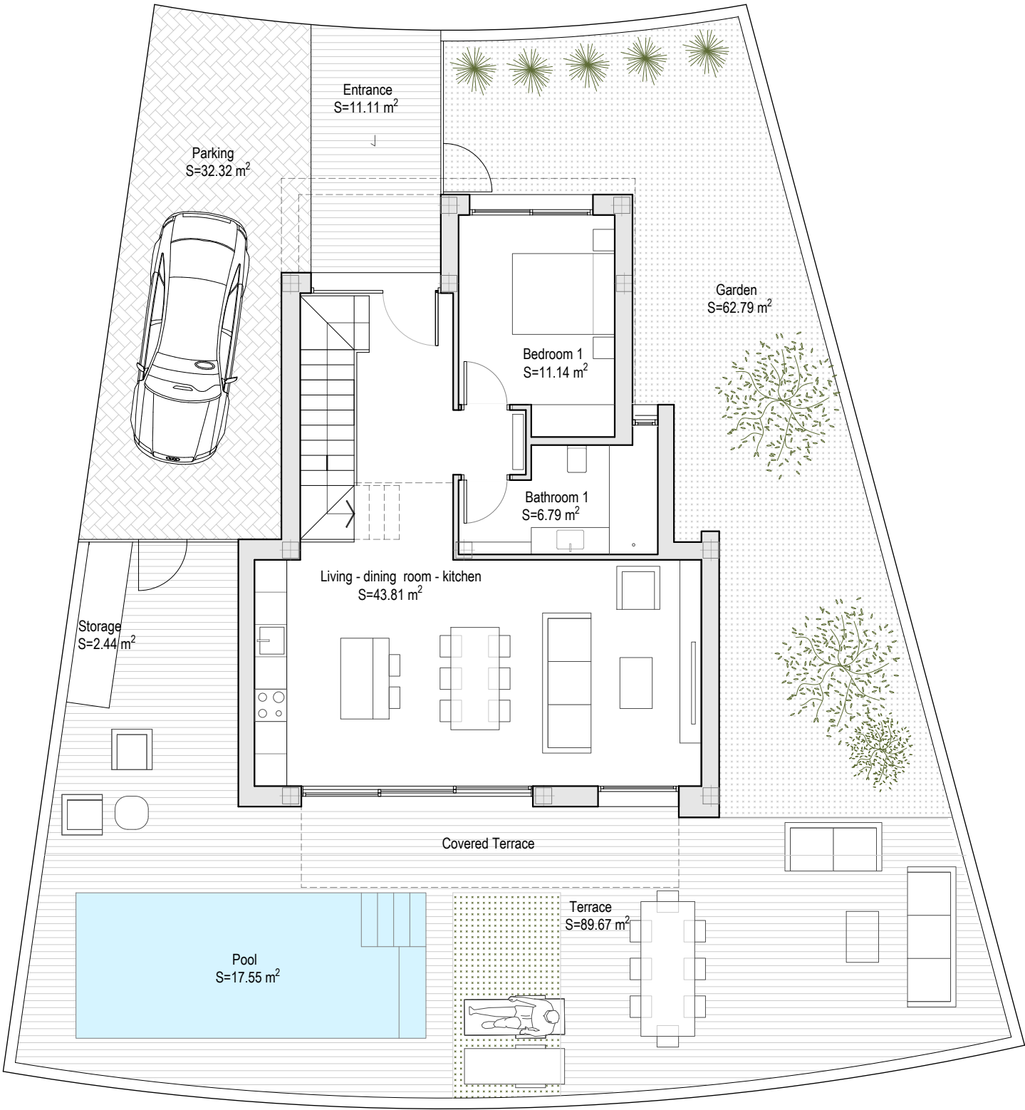
Ground floor
